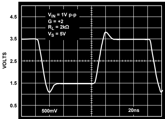
Figure 36. Large Signal Step Response; V_S = 5V , G = +2
