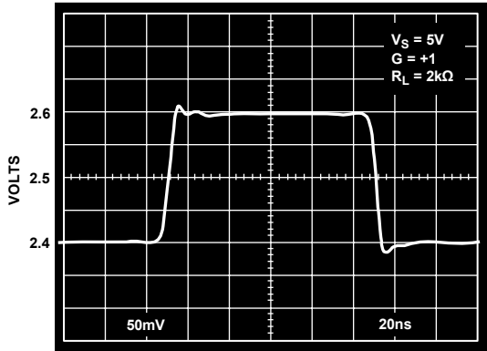
Figure 35. AD8051/AD8052 200 mV Step Response; V_S = 5V , G = +1
