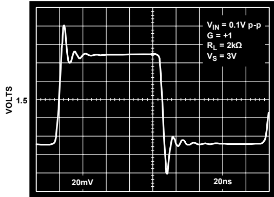
Figure 34. 100 mV Step Response, G = +1
